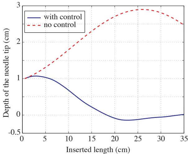
Fig. 7. Error in the parameter value: Initial deviation of x_1 = 10mm , \beta = 3^\circ and \gamma = 5^\circ . Error in the parameter value is 10%. Noise in the depth measurement taken to be within \pm 1mm . Notice that the controller stabilizes the needle tip to the desired location even when there is an error in the model parameter, \kappa .
