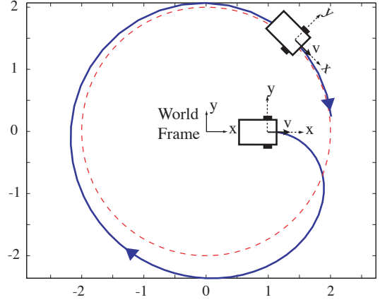
Fig. 1. Cart following a circle: Red dotted circle is the desired circle to be followed by the cart. Initially the cart is away from the desired circle but with the application of the controller, it follows the circle.
