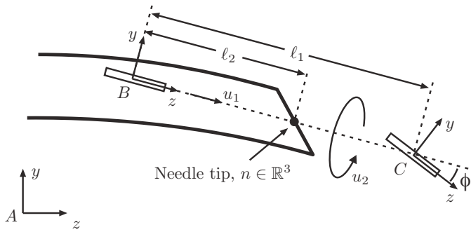
Fig. 2. Needle steering kinematic model: Frame A is the inertial world reference frame. Frames B and C are attached to the two wheels of the bicycle. This figure is reproduced from [16] with permission from the authors.
