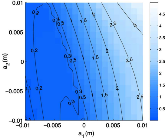
Fig. 10. Maximum nonunity eigenvalue for the linearized return map at various fixed-COP positions around the COM. Parameters used for P. americana are shown in the caption of Fig. 11.
