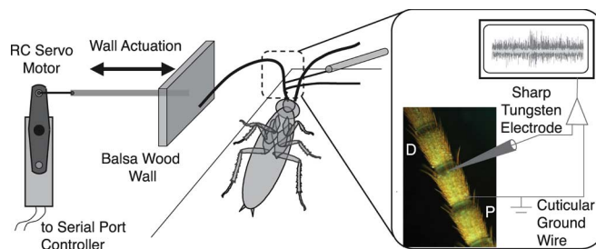
Fig. 3. Electroantennogram experimental setup: an RC servo motor drives a wall segment against the free antenna of a restrained cockroach simulating a 30^\circ turn during fast locomotion ( \sim 45 cm/s). A tungsten electrode provides extracellular recordings from the antennal nerve (darker trace in inset), which are significantly above noise (lighter trace). The zoomed photo of the antenna is an autofluorescent image of three flagellar segments taken under a green fluorescent protein (GFP) filter to highlight the mechanosensory hairs, the largest on each segment. The distal (D) and proximal (P) labels indicate orientation.
